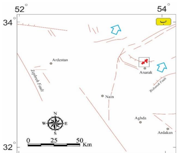
Direction of maximum horizontal shortening deduced from Neogene axes of folding City Thrust Fault(0-35°)
