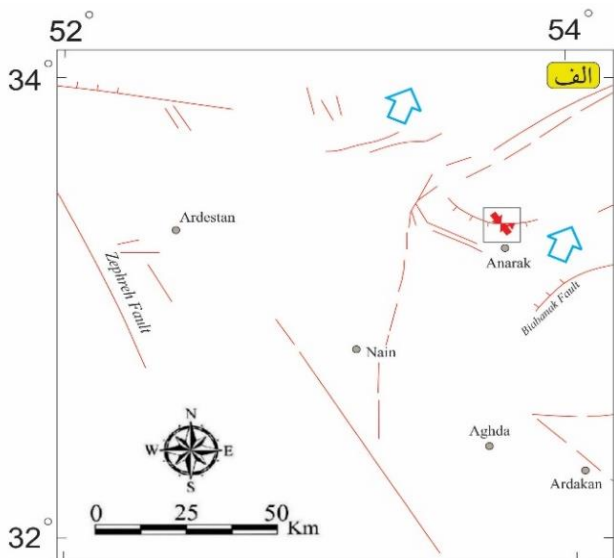
High angle reverse fault(36°-90°)
