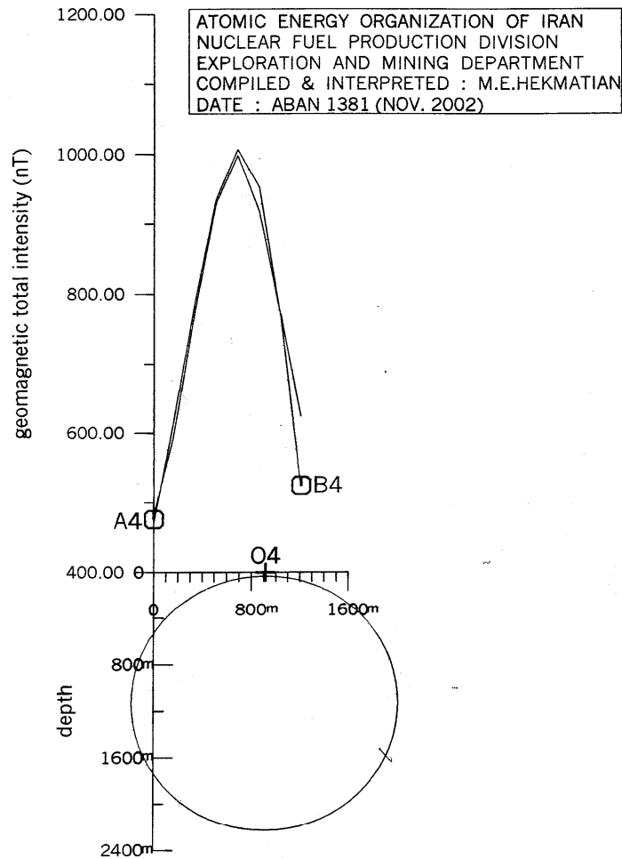
PROFILE A4B4 OF ANO1 (ABRIZ AREA)
